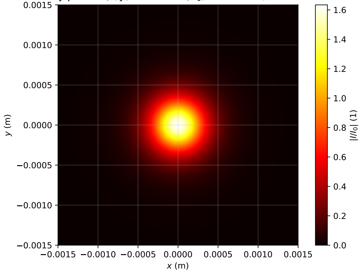
Intensity profile I(x, y, z = 2.070m)/I_0 , Pin=0.9Pcr, artificial time
